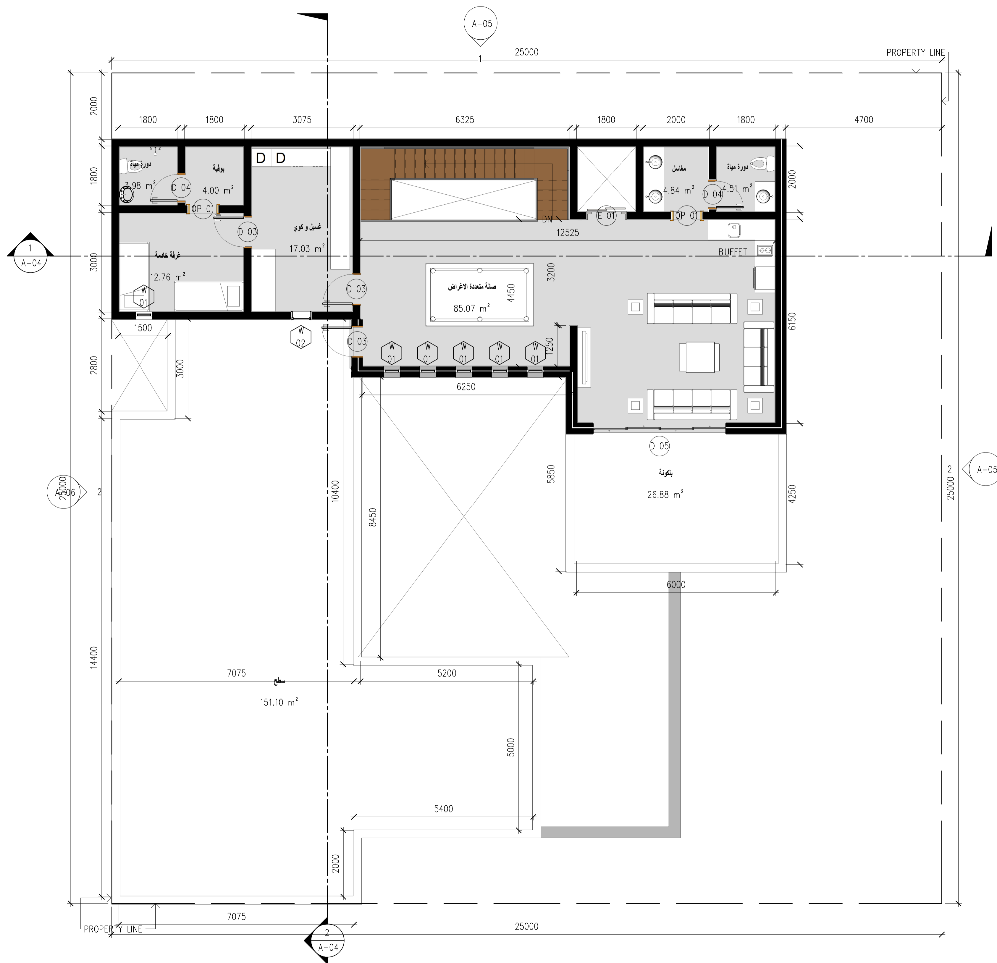
1 ROOF ANNEX FLOOR PLAN 1 : 100
