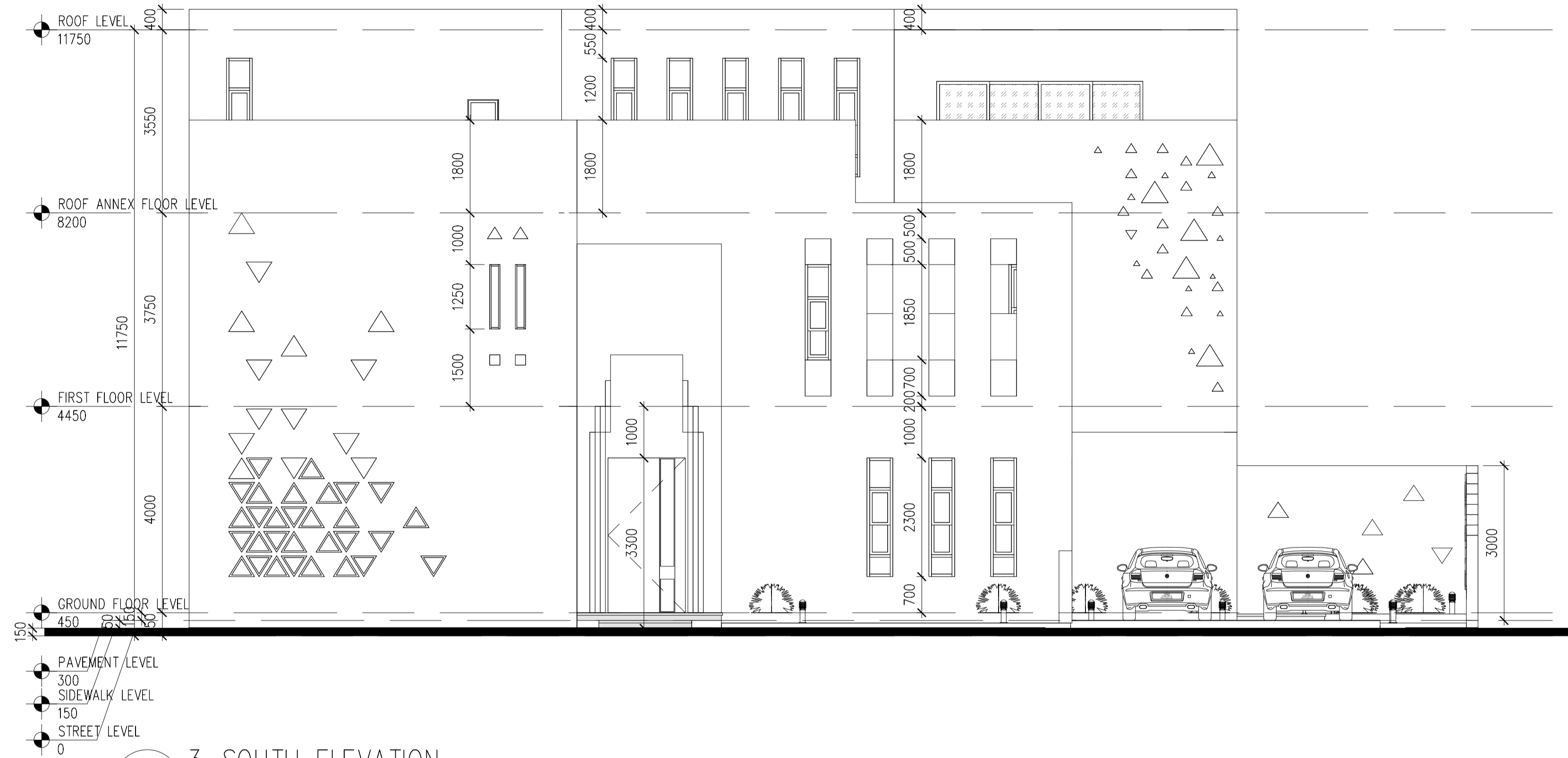
1 3-SOUTH ELEVATION 1 : 100
